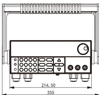
IT6722/IT6722ADimension figure
