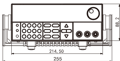
IT6723H/IT6724H/T6723GDimension figure
